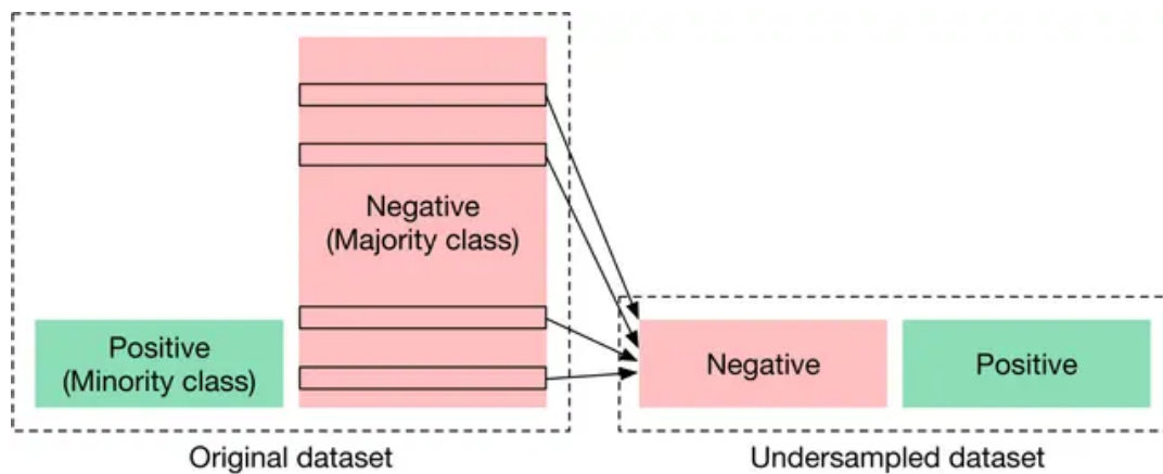
Figure 1.18: Undersampling the majority class
