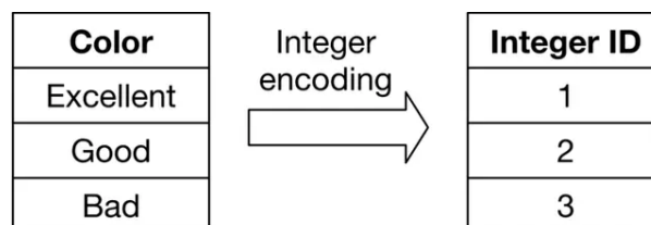
Figure 1.13: Integer encoding
