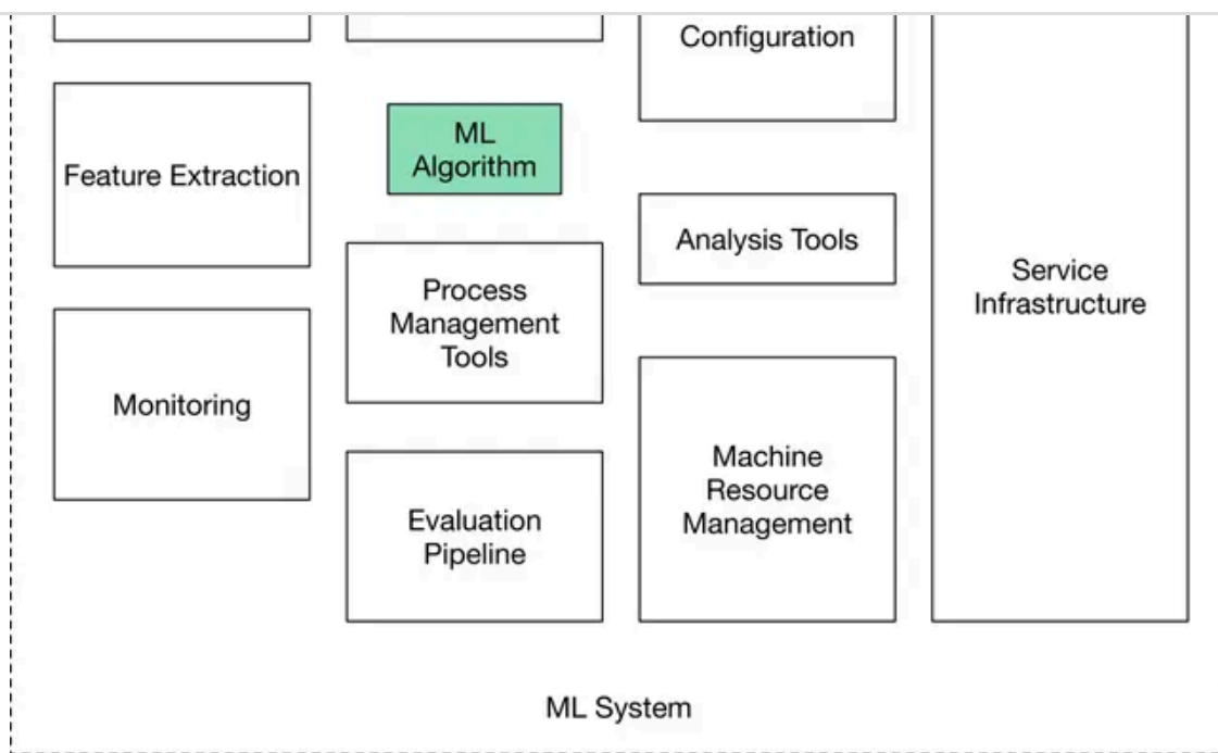
Figure 1.1 Components of a production-ready ML system
