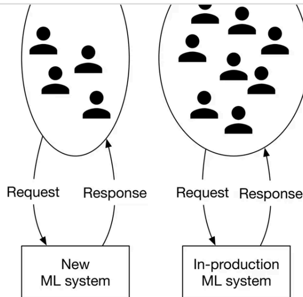
Figure 1.20: A/B testing
