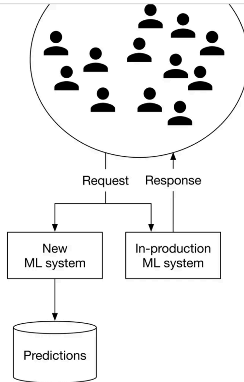
Figure 1.19: Shadow deployment
